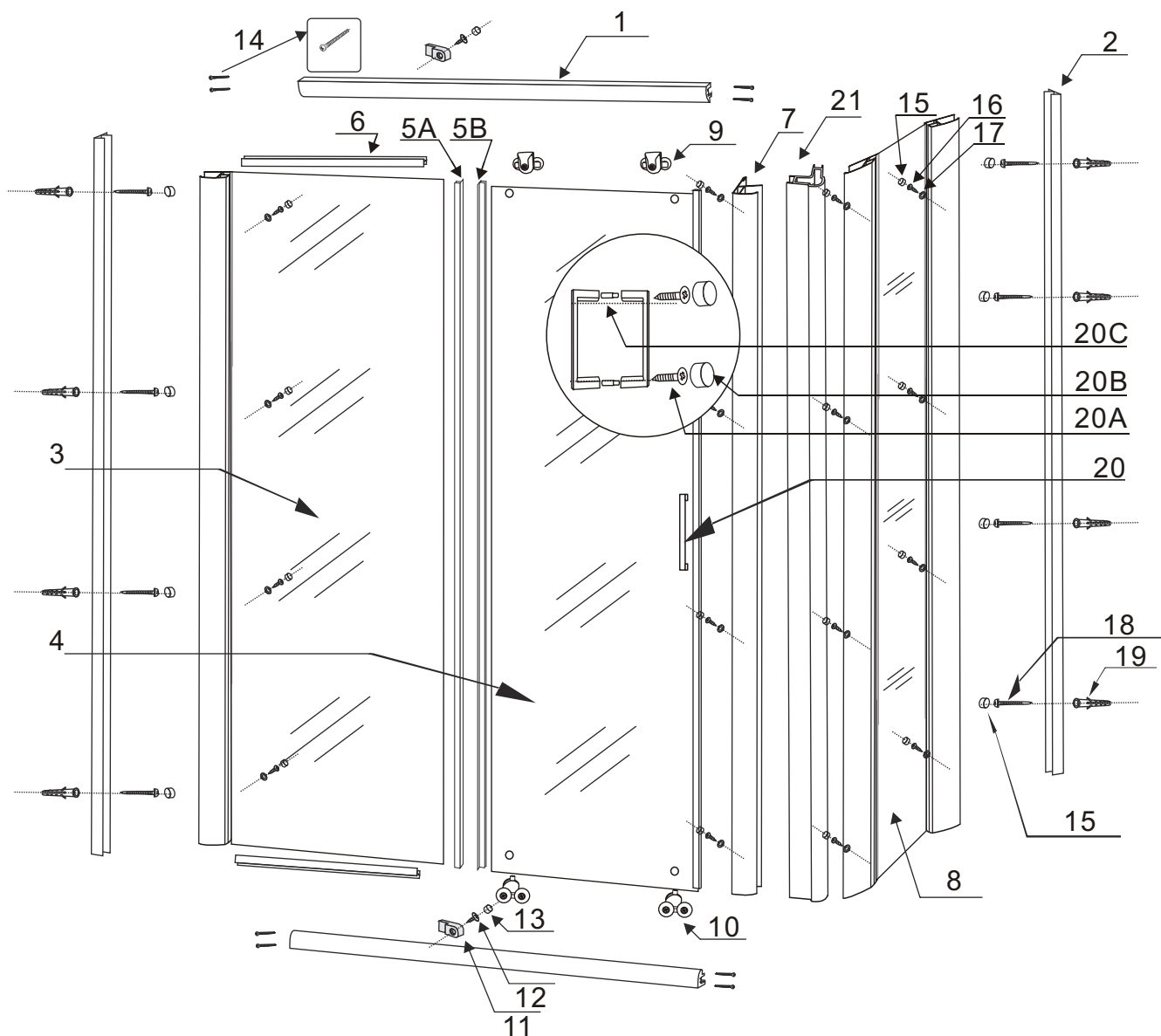
Sliding door with side panel
